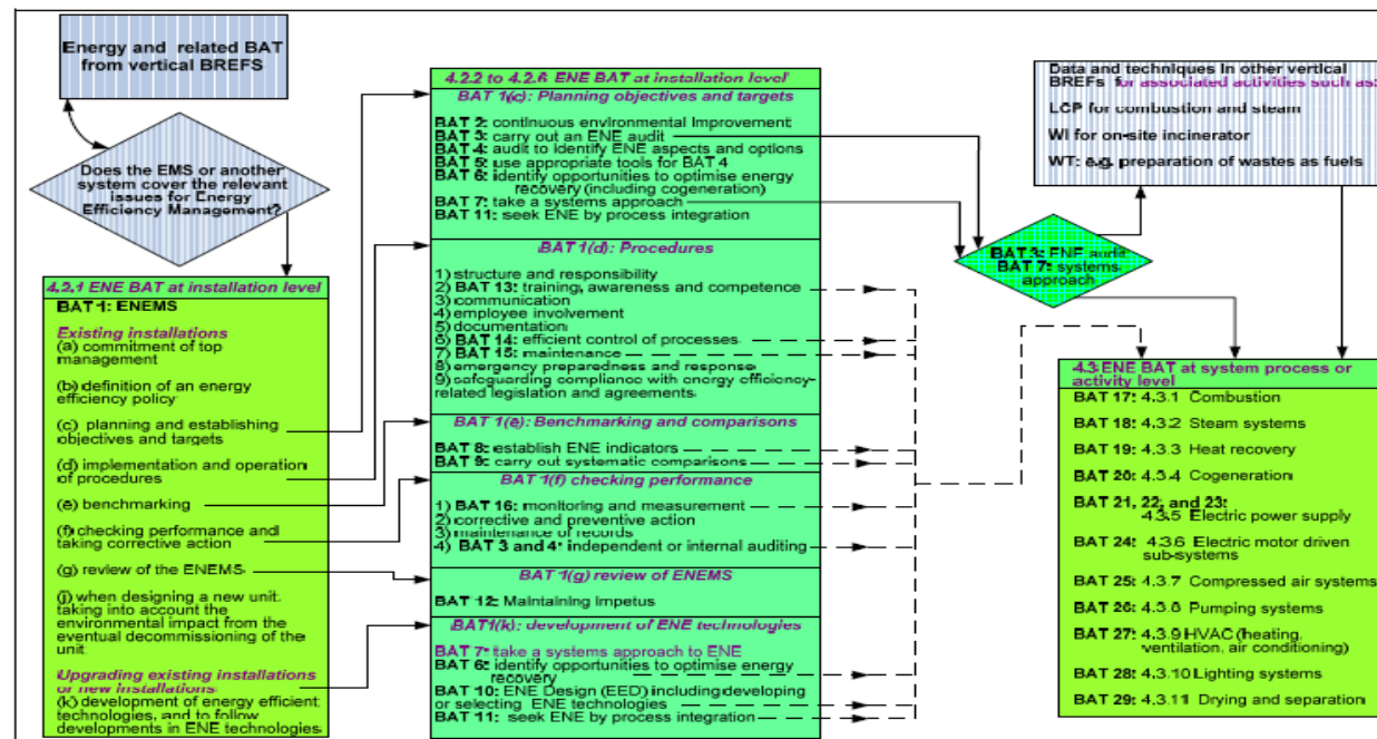
Figure 4.1: Relationships between BAT for Energy efficiency
